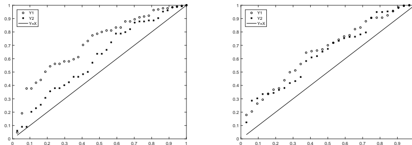
Figure 3: The scaled TTT plots of the marginals for data set 1 (Left), data set 2 (Right).
