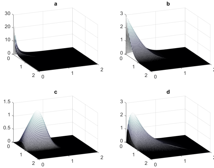
Figure 2: The shape of the joint probability density function of BCHG for different values of parameters \Theta = (\theta, \alpha, \lambda_0, \lambda_1, \lambda_2) : (a) \Theta = (0.5, 0.75, 2, 1, 1) (b) \Theta = (1, 1, 2, 1, 1) (c) \Theta = (2, 1.5, 2, 1, 1) (d) \Theta = (0.2, 1.5, 0.4, 0.4, 0.4) .
