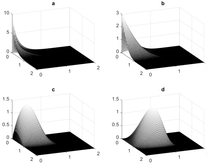
Figure 1: The shape of the joint probability density function of BCH for different values of parameters \Theta = (\alpha, \lambda_0, \lambda_1, \lambda_2) : (a) \Theta = (0.75, 2, 1, 1) (b) \Theta = (1, 2, 1, 1) (c) \Theta = (1.5, 2, 1, 1) (d) \Theta = (2, 0.7, 0.7, 0.7) .
