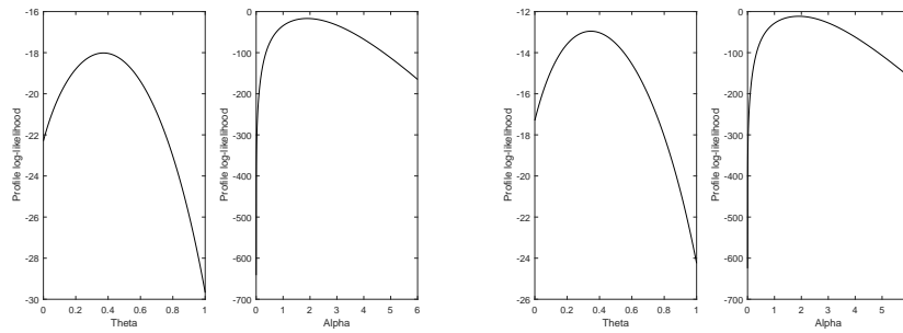
Figure 4: The profile log-likelihood function of \theta and \alpha for data set 1 (Left), data set 2 (Right).
